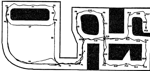
Figure 4-c. Exploration result with 10% sensor error
