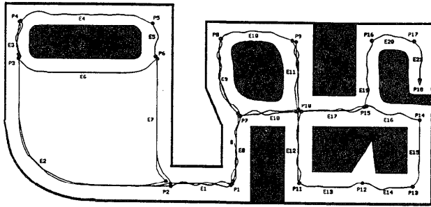
Figure 4-a. Exploration result with 0% sensor error
