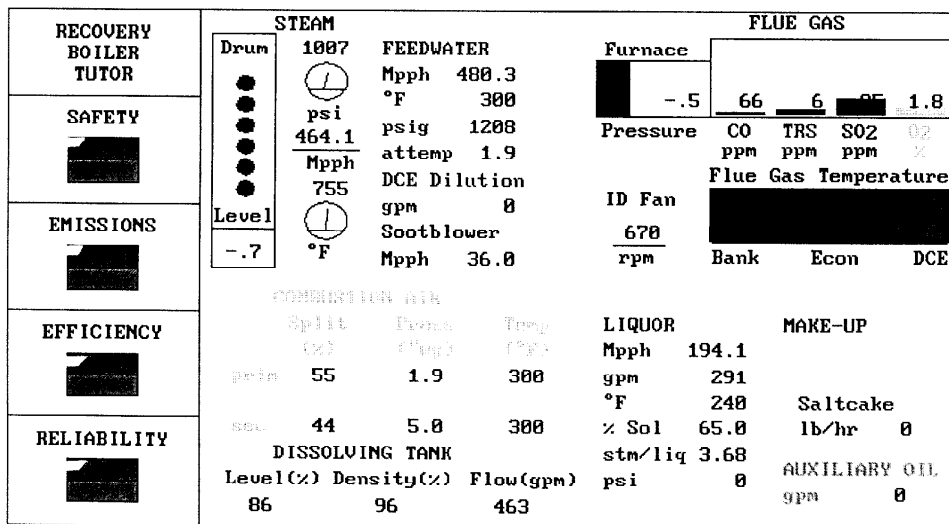
Figure 5: The Complete Control Panel.
