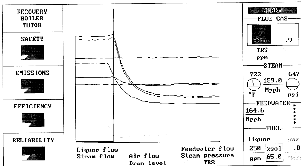
Figure 6: Trends Selected by the Operator.
