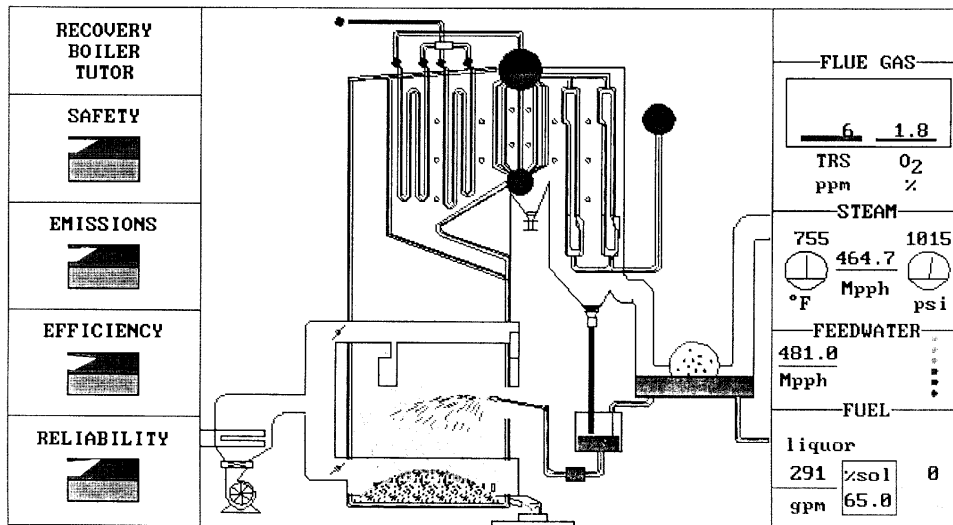
Figure 1: Sectional View of the Recovery Boiler.
