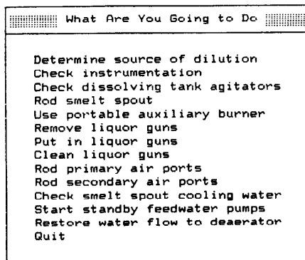
Figure 3: Menu to Select a Physical Task to Perform on the Boiler.
