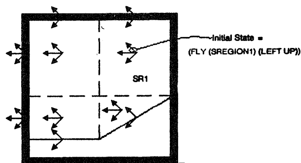
Fig. 5. A Sequence Graph
