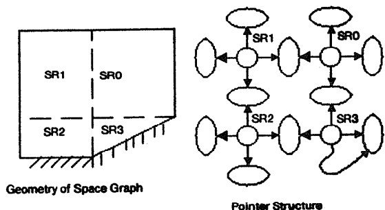
Fig. 2. Space Graph for a scene
